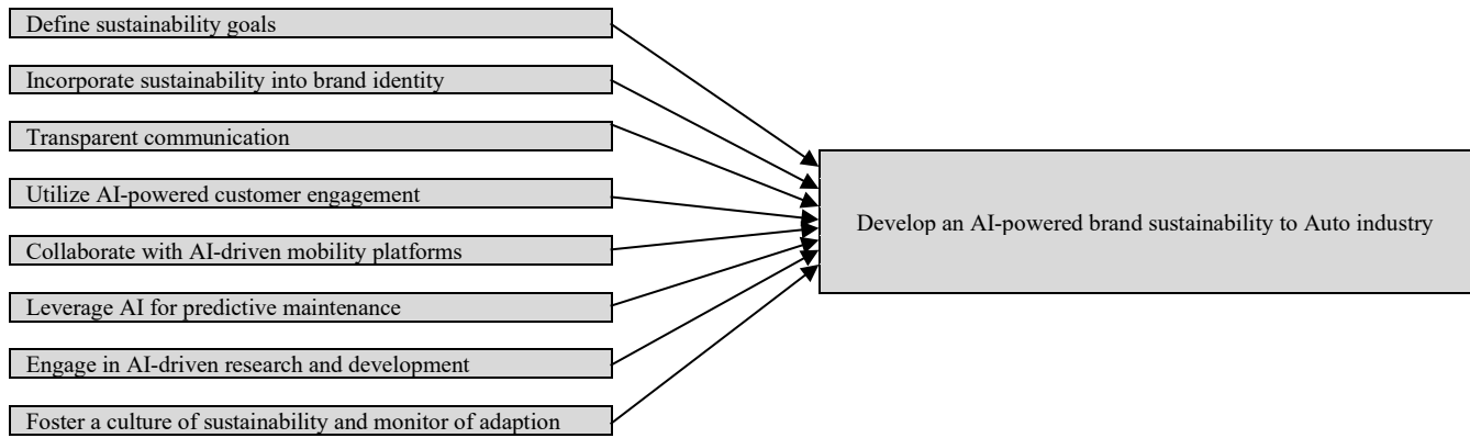
Fig. 1. Hypothesis model
