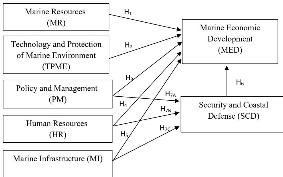
Fig. 1. Research model
